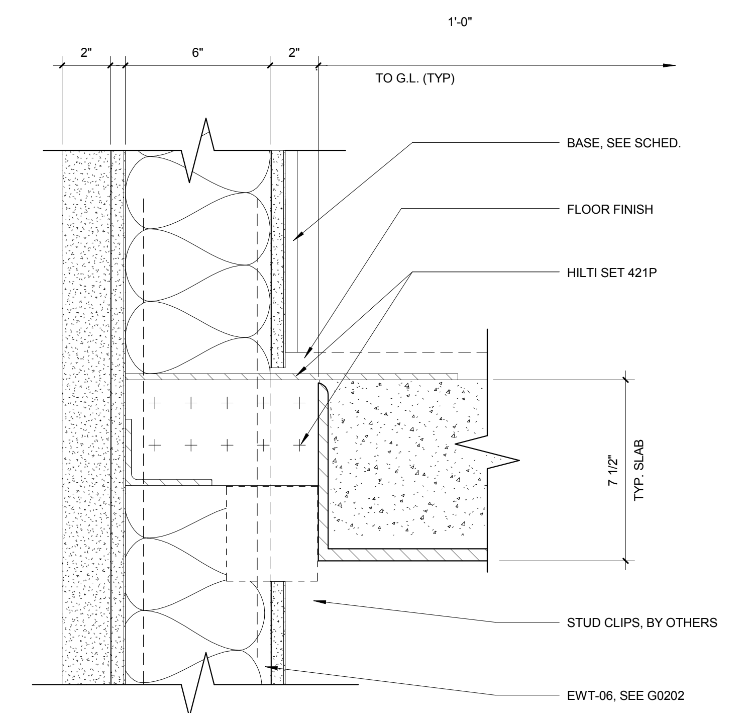
1 TYP. EDGE OF SLAB A7114 3/8" = 1'-0"
