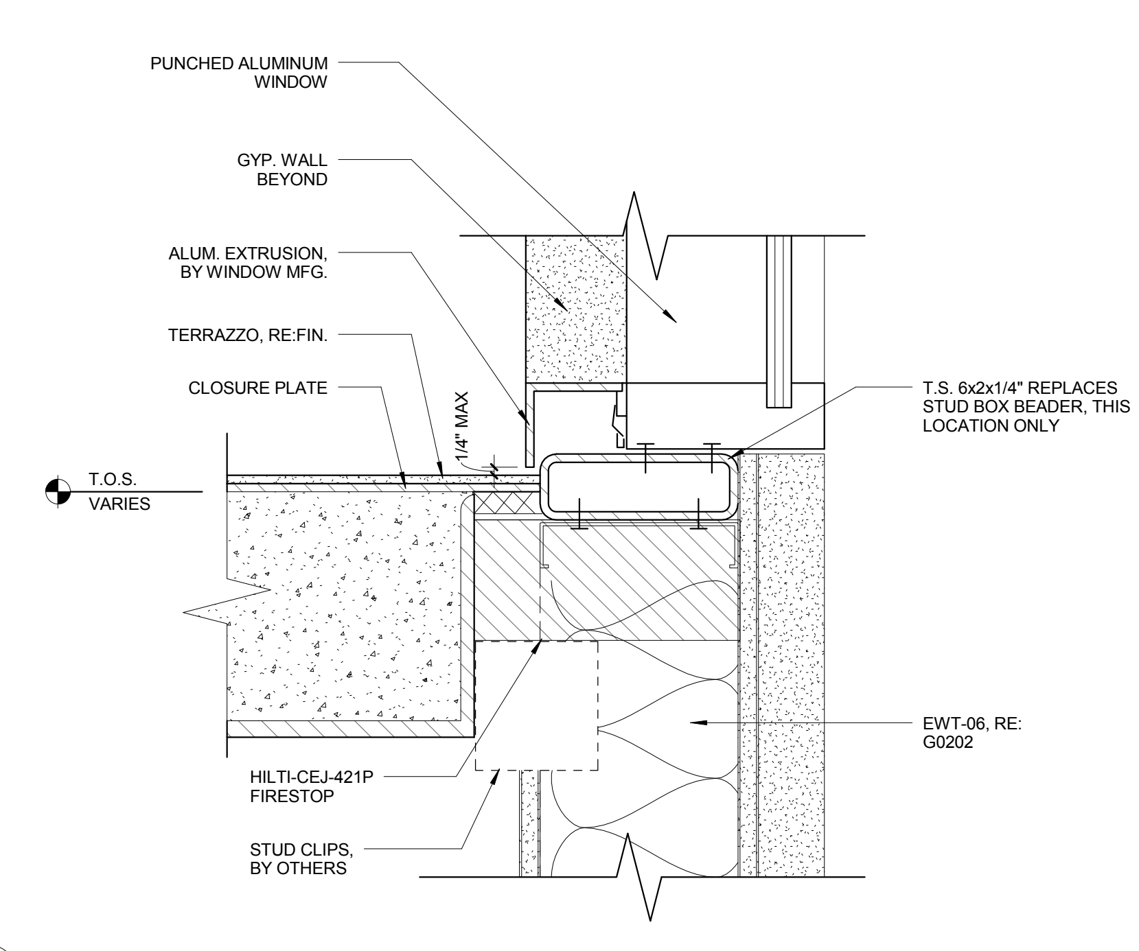
2 DETAIL A7114 3/8" = 1'-0"
